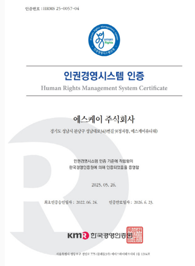
HRMS
